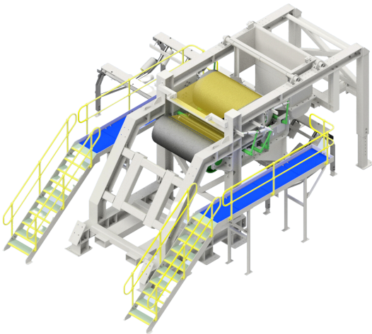
DEVELOPMENT CONVEYOR TRANSFER DESIGNED, ENGINEERED AND DRAFTED BY RED ENGINEERS
