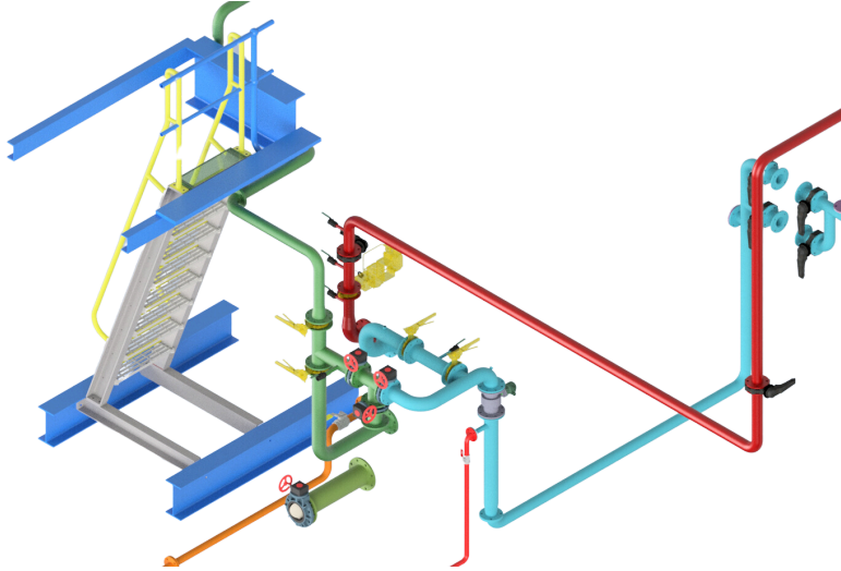
REMELT SYSTEM DESIGN - MACKAY SUGAR DESIGNED, ENGINEERED AND DRAFTED BY RED ENGINEERS
