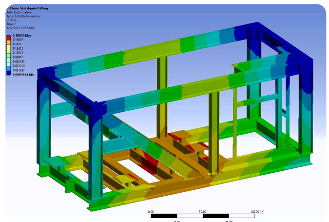
TRANSPORT FRAME - ENGINEERING ASSESSMENT DESIGNED, ENGINEERED AND DRAFTED BY RED ENGINEERS
