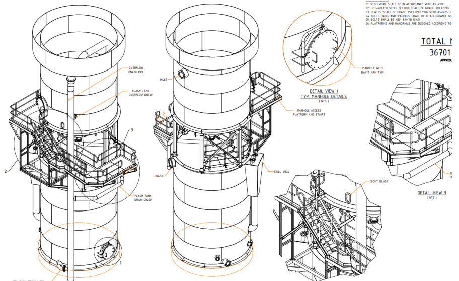
ESJ TANK - MACKAY SUGAR - DESIGNED, ENGINEERED AND DRAFTED BY RED ENGINEERS
