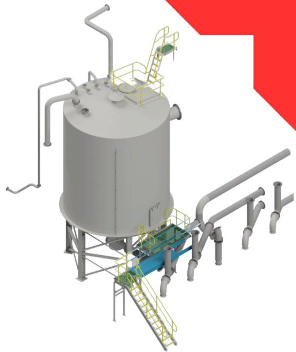
PRIMARY JUICE TANK - MACKAY SUGAR - DESIGNED, ENGINEERED AND DRAFTED BY RED ENGINEERS
